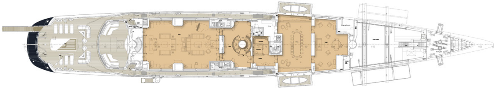
Main Deck
