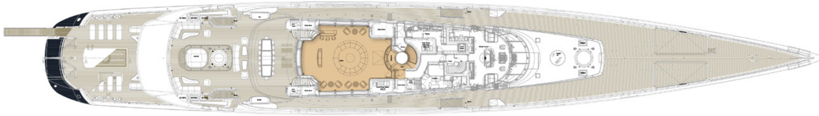
Upper Deck
